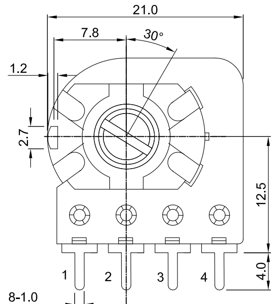
Shaft shown in full C.C.W. position
