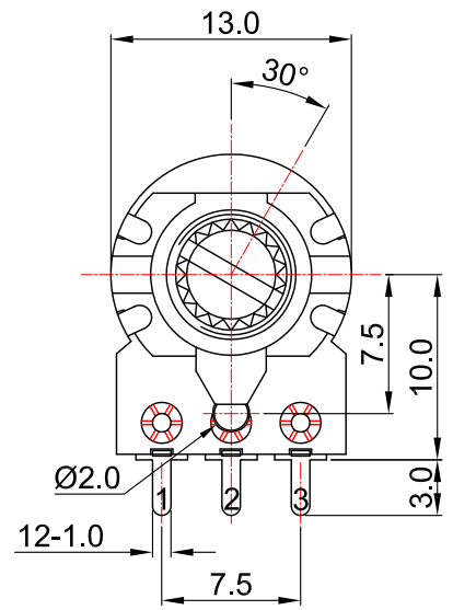
Shaft shown in full C.C.W. position
