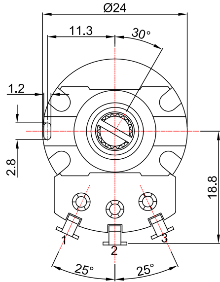
Shaft shown in full C.C.W. position
