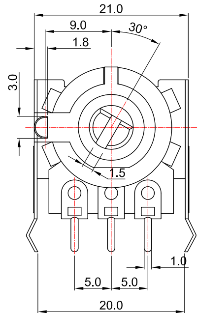
Shaft shown in full C.C.W. position
