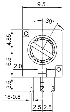
Shaft shown in full C.C.W. position
