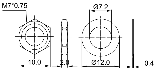
Attached parts: nut & washer
