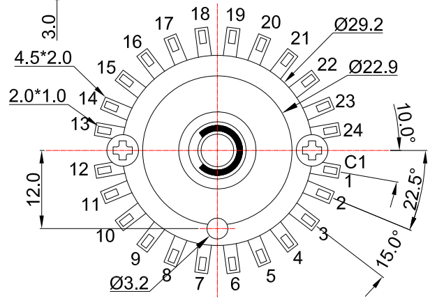
Shaft shown in full C.C.W position
