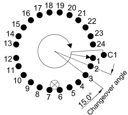
Shaft shown in full C.C.W position
